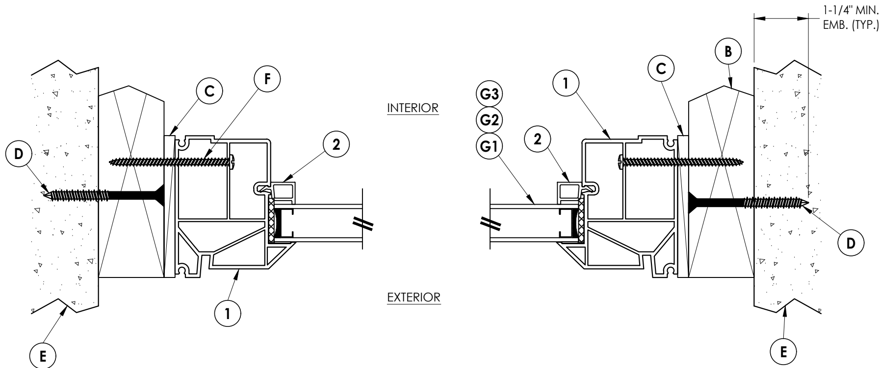
1 HORIZONTAL CROSS SECTION 2 2X Buck Masonry Construction
