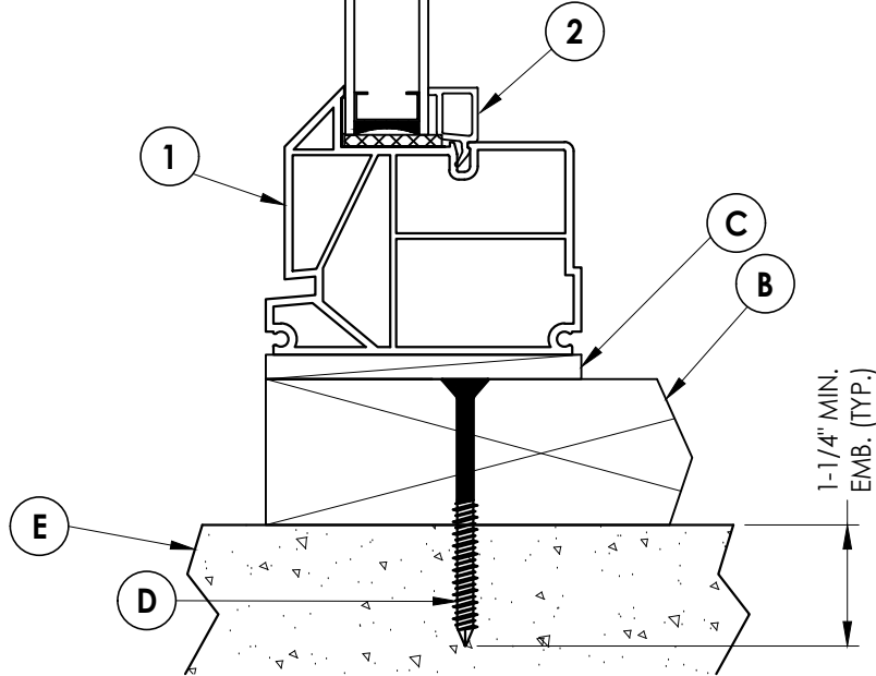
2 VERTICAL CROSS SECTION 2 2X Buck Masonry Construction
